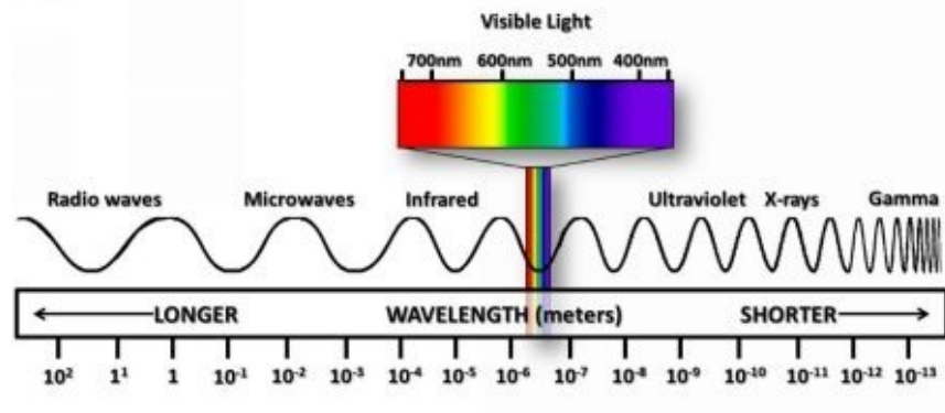
Figure 10: Electromagnetic Spectrum
